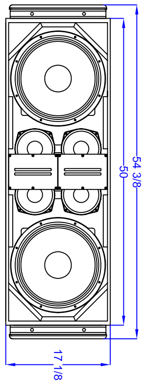
FRONT
